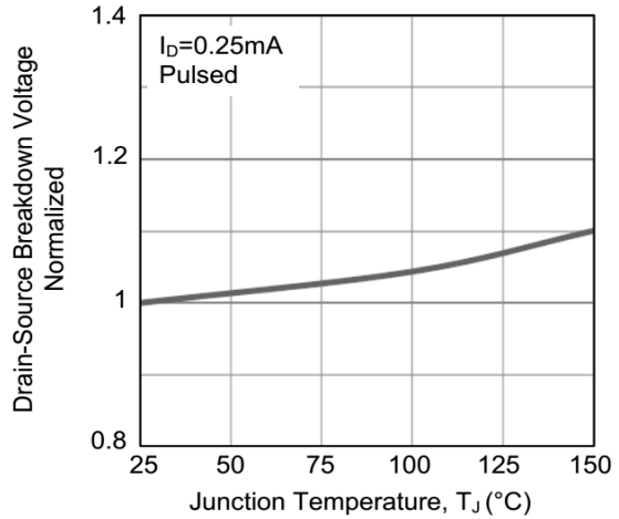
2. Breakdown Voltage vs. Junction Temperature
